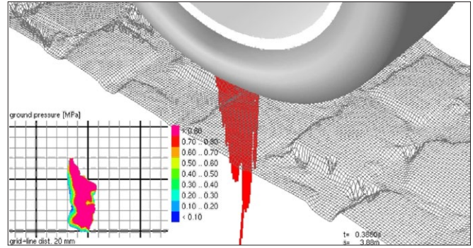
Rough road modeling
