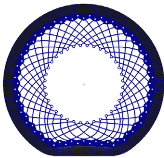
Non-pneumatic tire with composite springs
