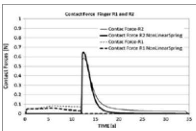
Figure 8. Finger contact force from simulation
