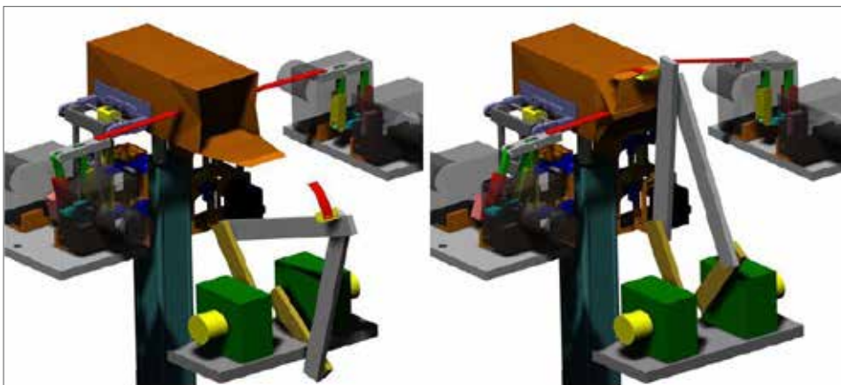
Figure 3. 3D Adams simulation for package folding machinery
