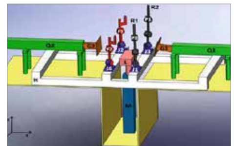
Figure 7. D-RAPS model created with Adams
