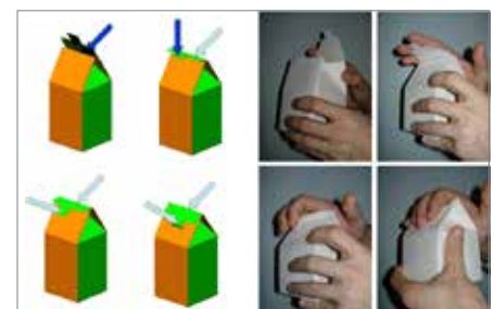
Figure 2. Tuck-in operation by human fingertip and kinematic analysis. From top left to the bottom right: a) first flap folding, b) second flap folding, c) the third flap folding, d) the tuck-in of the third flap.
