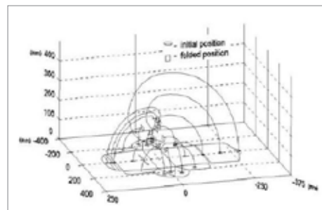
Figure 6. Carton folding trajectories for more complex folding operation
