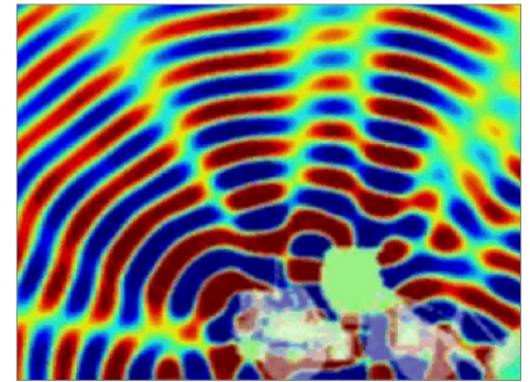
Actran results: sound propagation (phase) at blade-pass frequency
