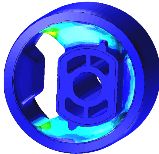
Large strain simulation of a rubber bushing using the adaptive load stepping scheme
