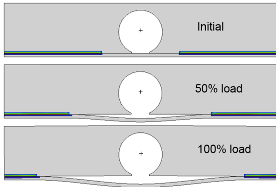
Crack propagation using VCCT
