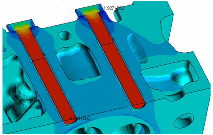
Bolt pre-tension simulation using body contact with friction
