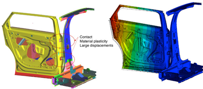
SOL400 simulation of partial car body & rear door, image courtesy of PSA
