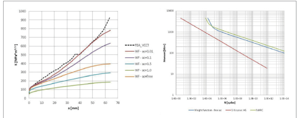
Crack growth approach, with weighing function and VCCT method, shows longer life for cylinder with notch. In the curve on the right, both crack growth and S-N results are plotted in an S-N diagram.
