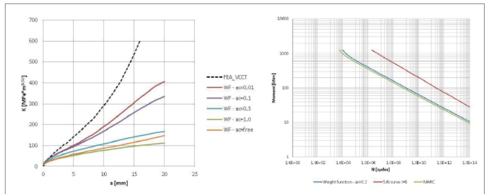
The plot on the left side shows the crack driving force on the y axis and the crack depth on the x axis for the VCCT and weight function approaches. The plot on the right shows the VCCT and weight function fatigue results compared with the S-N result.
