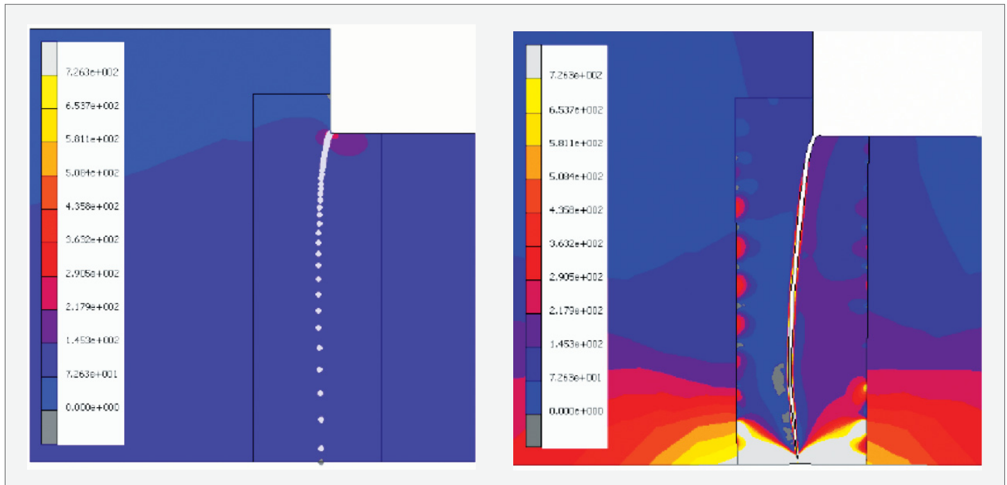
Predicted crack growth paths for notched cylinder, where the crack grows from the outer diameter.
