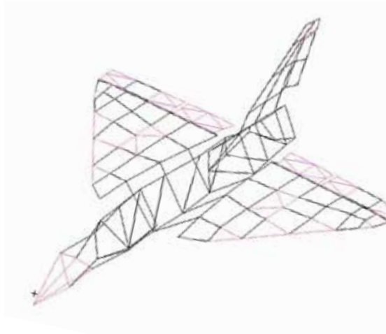
FE model of the aircraft generated from accelerometer locations in GVT
