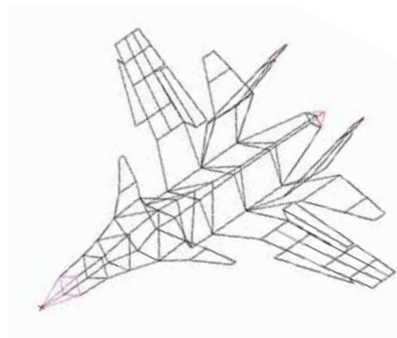
Dummy finite element model of aircraft requiring flutter clearance
